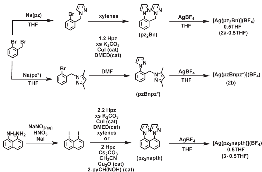
Scheme 1. Syntheses of Dipyrzolyloxyanils and Their Silver(I) Complexes
