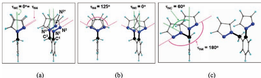
Figure 3. Two spacer-independent torsion angles, \tau_{N4} ( N^2N^1-N^1/N^2 , pink) and \tau_{NC} ( N^1C^1-C^3N^1 , green), for describing the relative conformations of pyrazolyls using pz_2Bn with coplanar pyrazolyls as an example (two views of the molecule are given for each conformation): (a) eclipsed, syn\text{-}\tau_{N4} = \tau_{NC} = 0^\circ ; (b) eclipsed, anti\text{-}\tau_{N4} = 125^\circ , \tau_{NC} = 0^\circ ; (c) staggered, anti\text{-}\tau_{N4} = 180^\circ , \tau_{NC} = 60^\circ . See the text for comments on the carbon hybridization.
