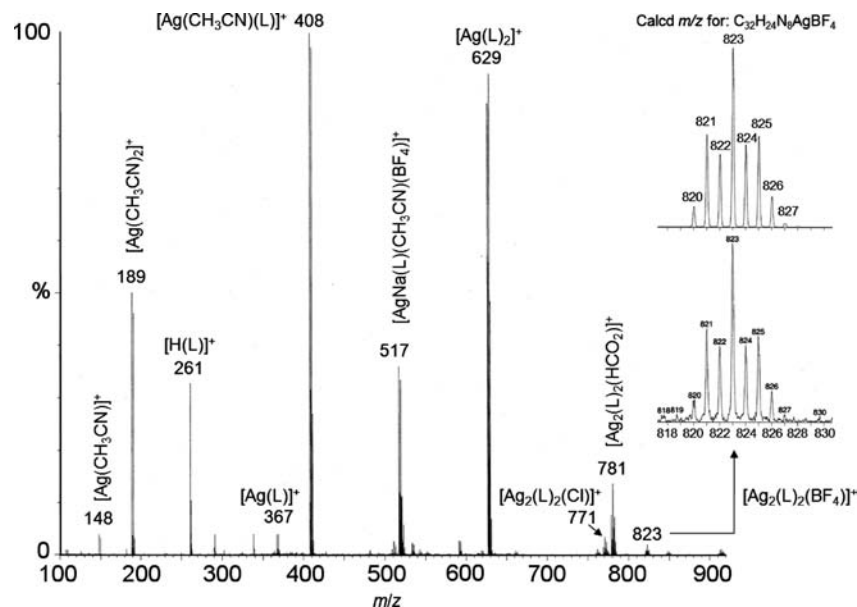
Figure 11. Representative ESI(+)-MS of 3 \cdot 0.5\text{THF} in acetonitrile.
