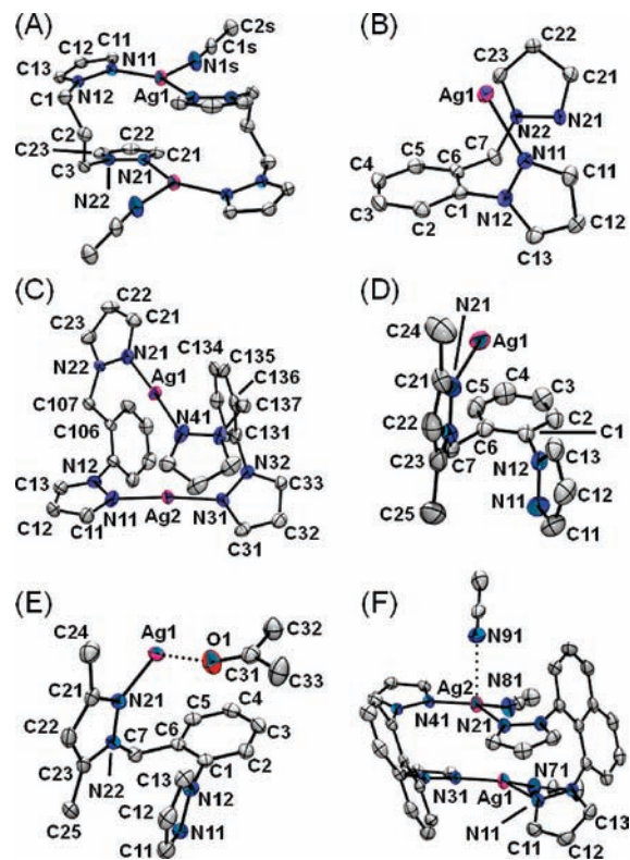
Figure 4. ORTEP diagrams (thermal ellipsoids drawn at the 50% probability level) and atom labeling of cyclic disilver dicationic or monomeric cation units of silver coordination polymers. (A) 1 · CH_3CN ; (B) 2a ; (C) 2a ·0.5acetone; (D) 2b ; (E) 2b ·acetone; (F) 3 · 2CH_3CN .
