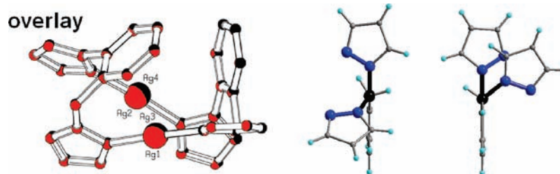
Figure 7. Overlay of two crystallographically independent cyclic dications in 2a ·0.5acetone (left) with views of gauche,syn (center) and staggered,syn (right) ligand conformations that occur within each cyclic dication.
